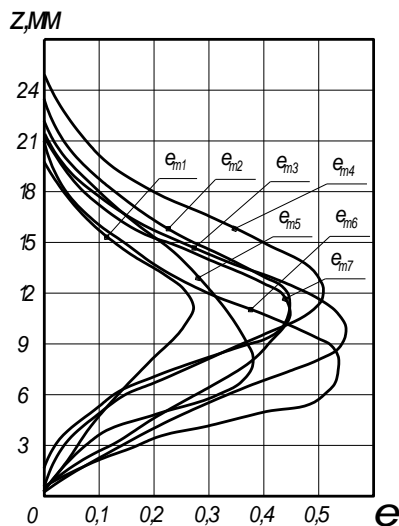
Fig. 4. Distribution of the main logarithmic deformation in the longitudinal direction of the piston after rolling (internal cavity)
